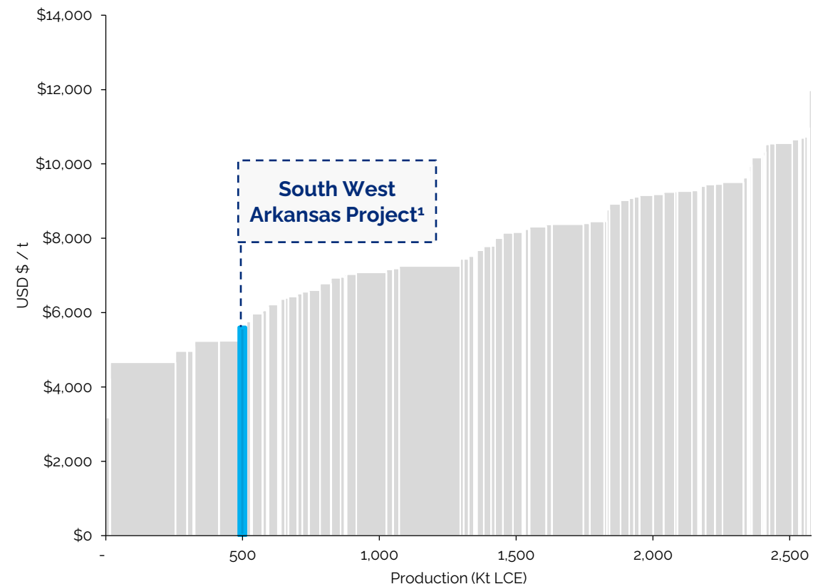
GLOBAL LITHIUM PRODUCTION COST CURVE³
